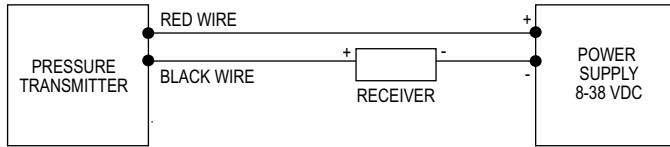
2-wire connection
