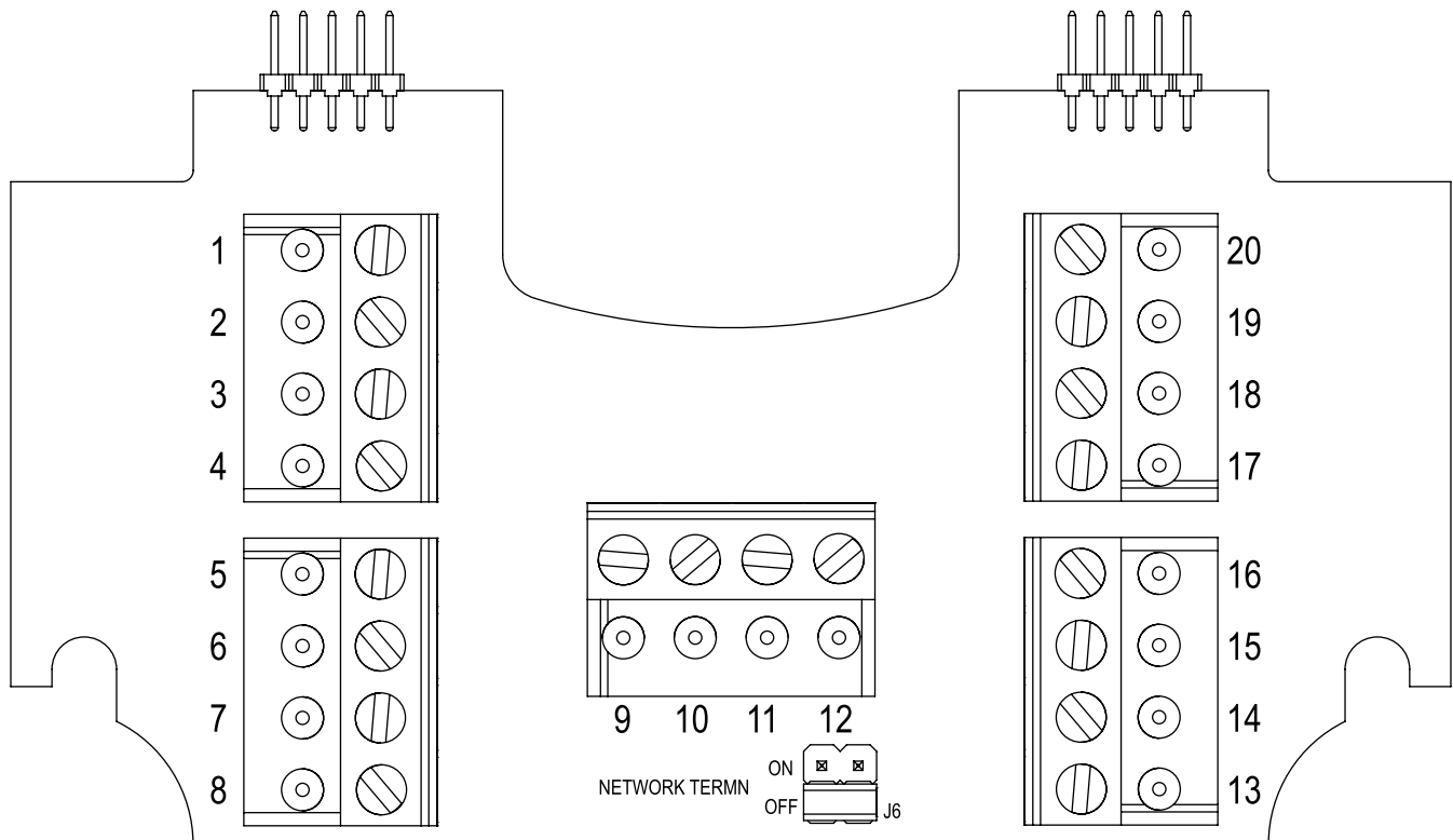
Figure 18: PCBA
