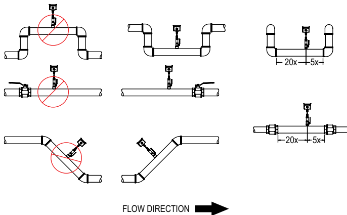
Figure 4: Proper installation location
