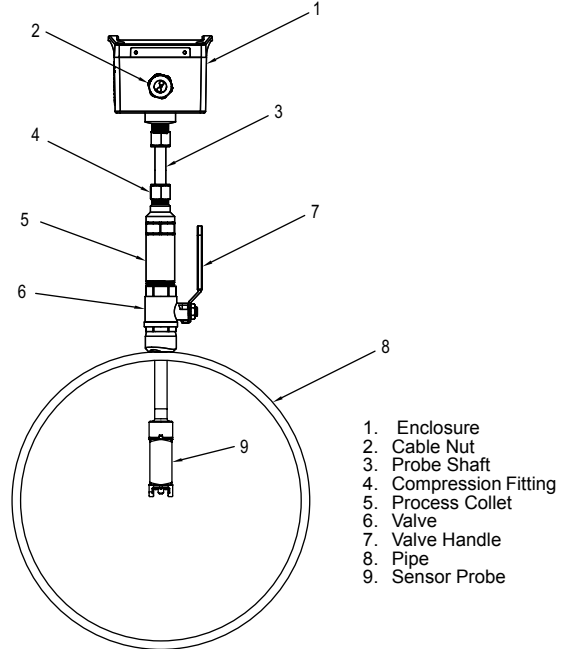
Figure 22: IEFB Side System View
