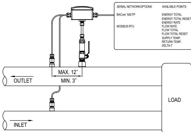
Figure 1: Typical installation
