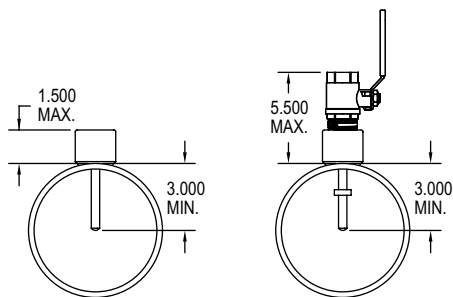
Figure 13: Stack height
