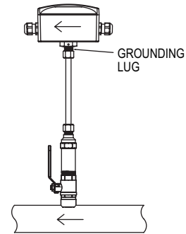
Figure 16: Metallic grounding
