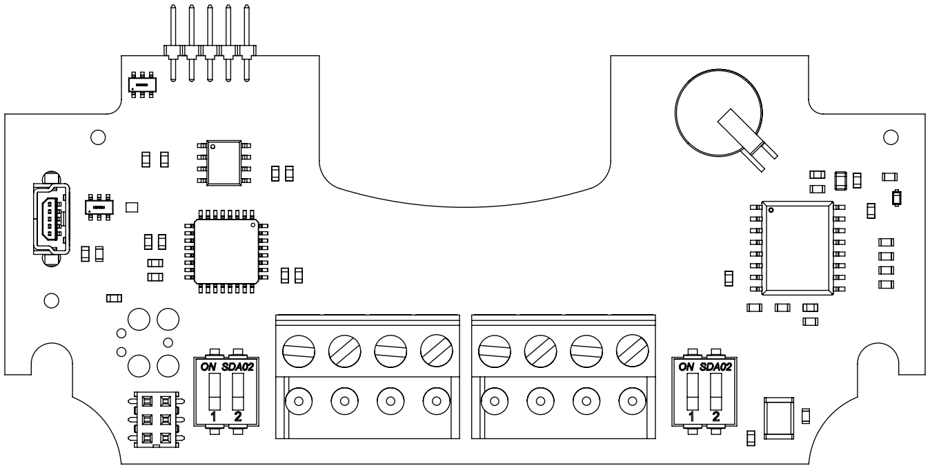
Figure 19: PCBA
