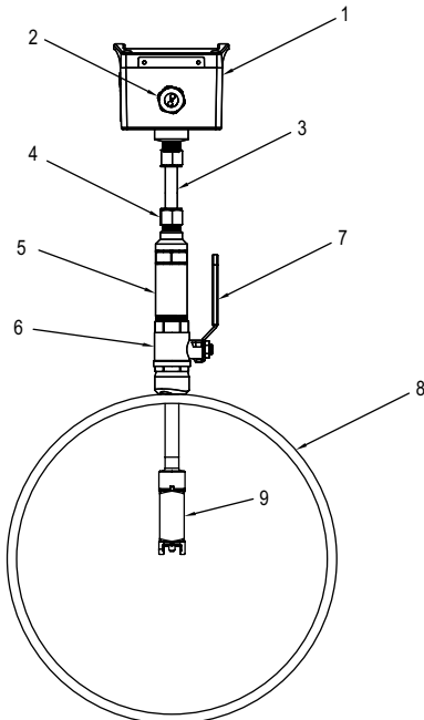
Figure 8: Side system view
