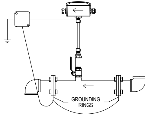
Figure 17: Non-metallic grounding
