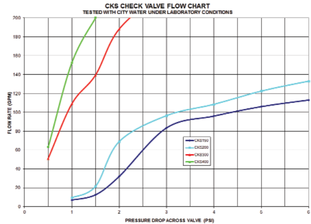
Typical data, actual may vary due to spring force variation.
