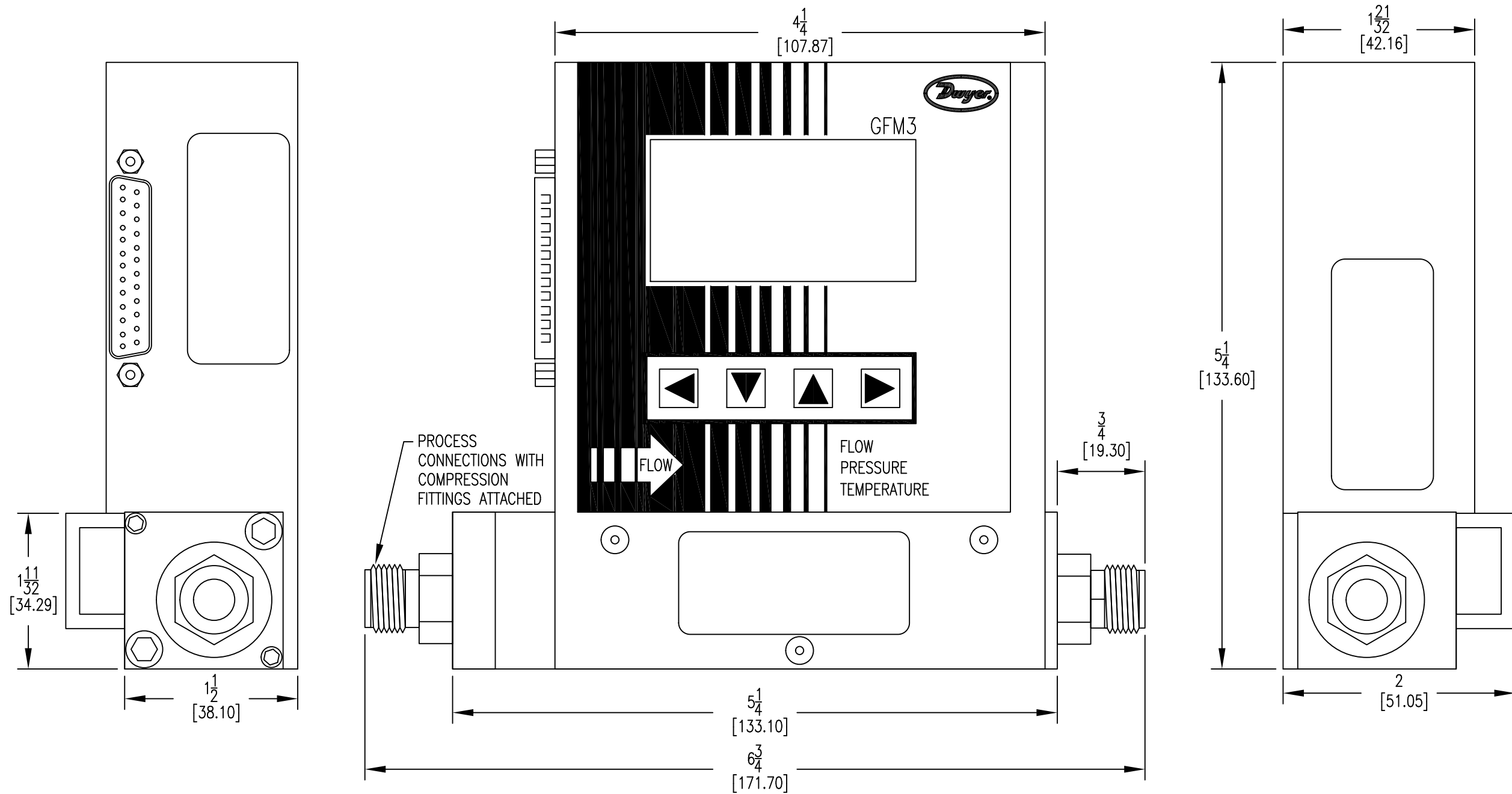
FLOW METER
